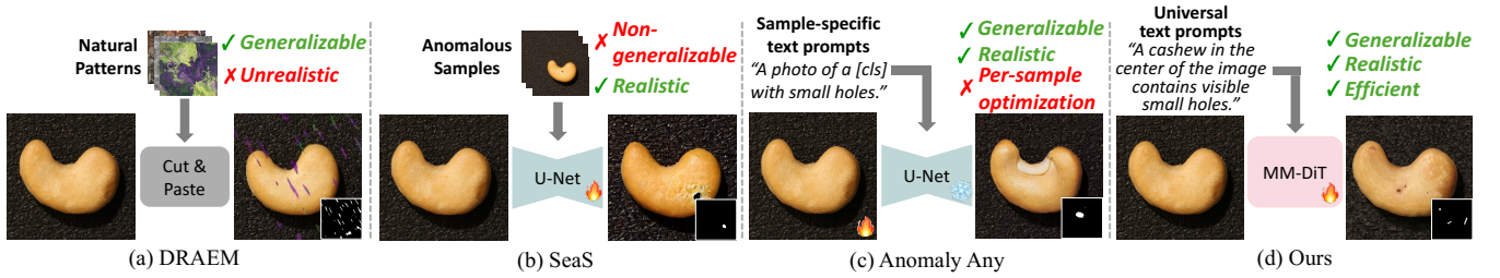
Figure 1: Comparison of Anomaly Generation Methods. (a) DRAEM uses cut-and-paste augmentation with natural patterns, offering generalizability but resulting in unrealistic anomalies. (b) SeaS leverages Stable Diffusion with anomalous exemplars, producing realistic samples but lacking generalizability. (c) Anomaly Any uses sample-specific prompts, achieving realism and generalizability but requiring costly per-sample optimization. (d) Ours introduces universal, structured text prompts to guide Stable Diffusion, enabling anomaly generation that is realistic, generalizable, and efficient.
