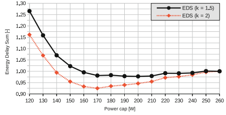
Fig. 5. EDS ( k = 1.5 and k = 2.0 ) vs power cap – 8 GPUs
